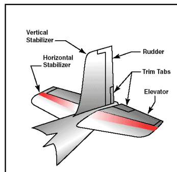
Figure 2: Empennage components.
